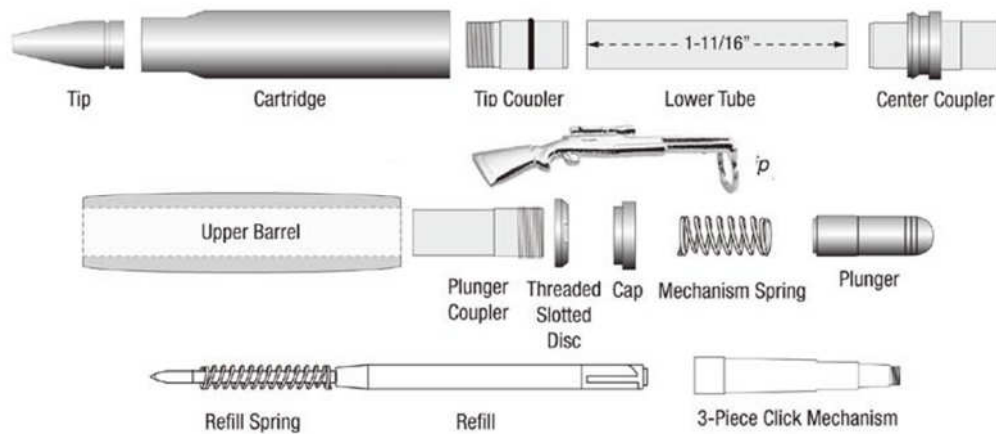
DIAGRAM C • Assembly
